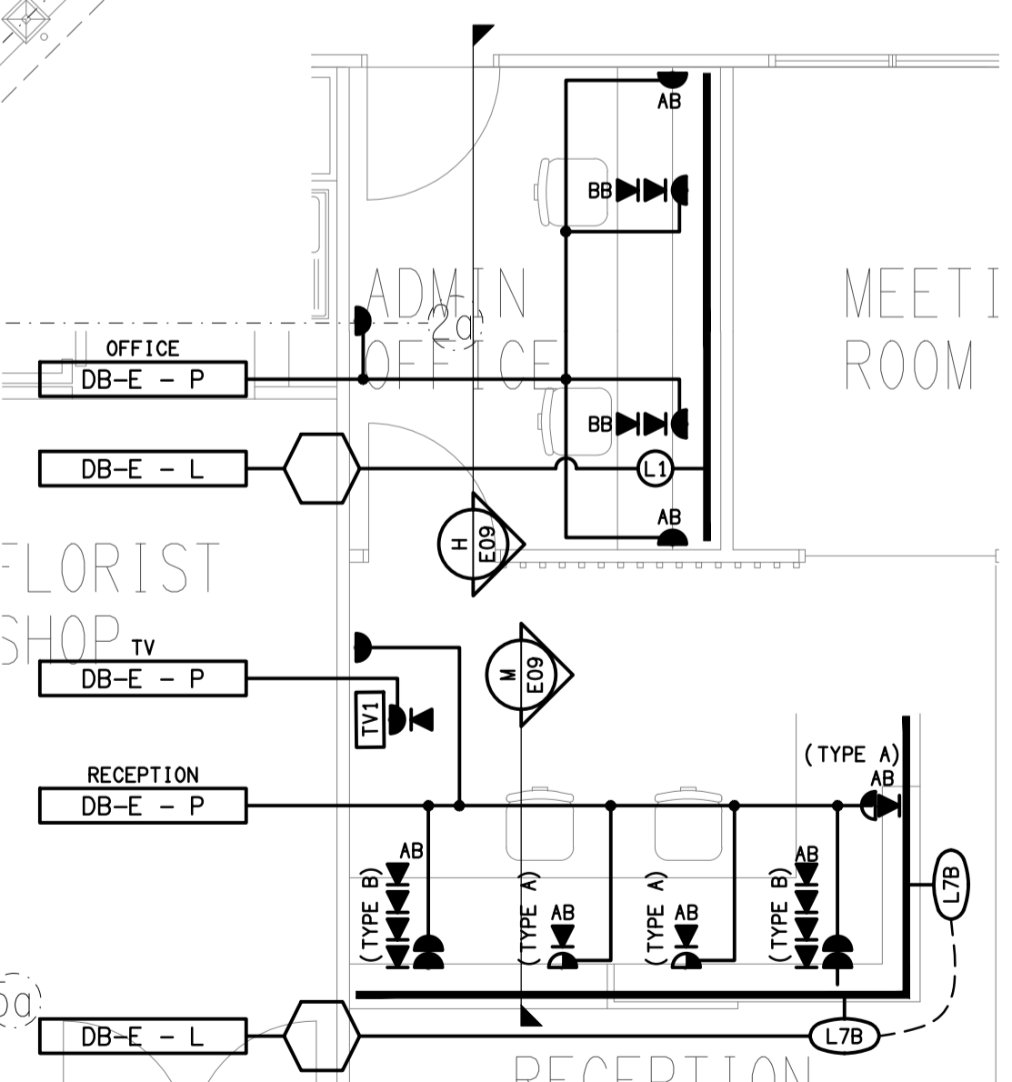
DETAIL A ADMIN OFFICE & RECEPTION SCALE 1:50
